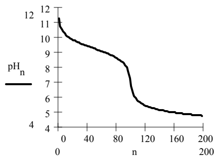
Fig. 3.1. Titrarea BS cu AS ( \text{NH}_3 cu \text{CH}_3\text{COOH} )
